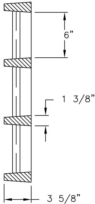
GRATE SECTION
