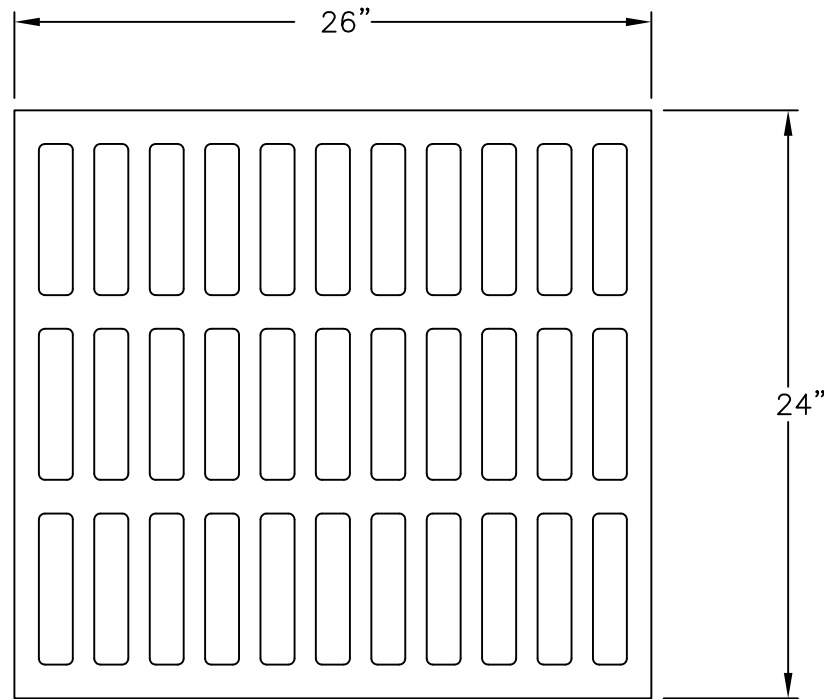
GRATE TOP VIEW
